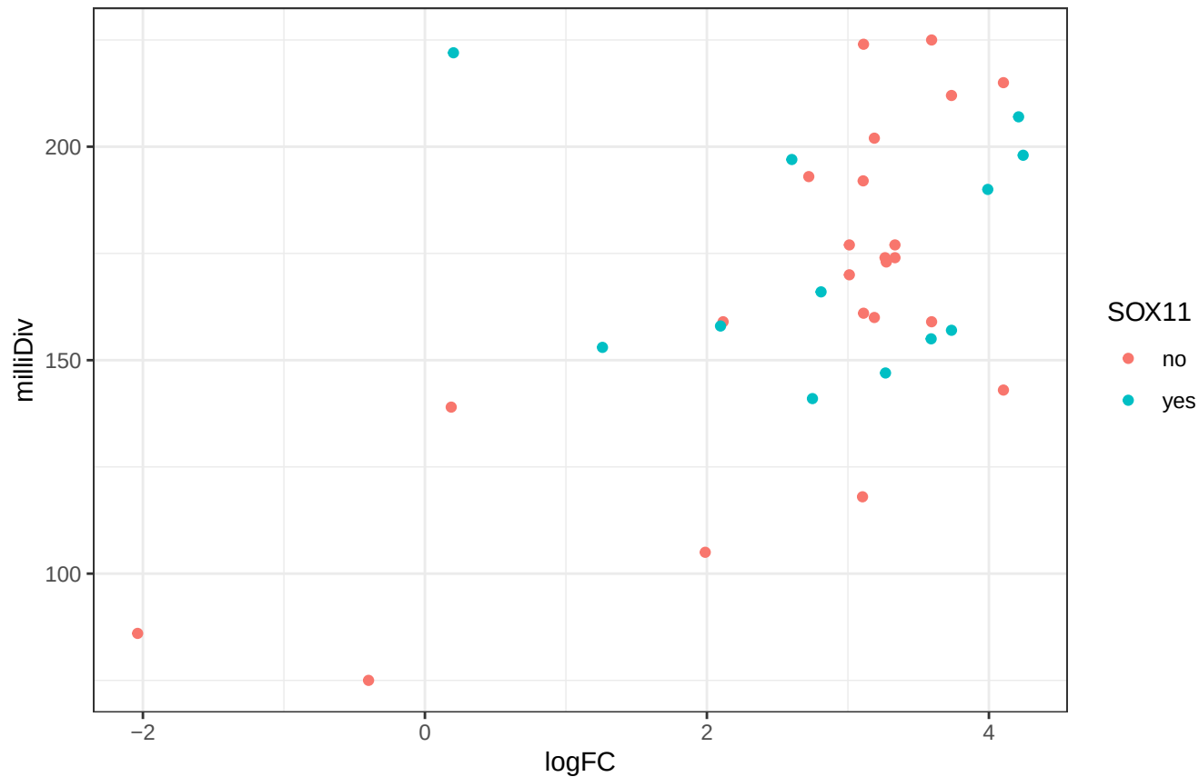
H3K27ac logFC at 0R which overlap a LTR10E and the milliDiv of the LTR10E, n=35 colored for SOX11
